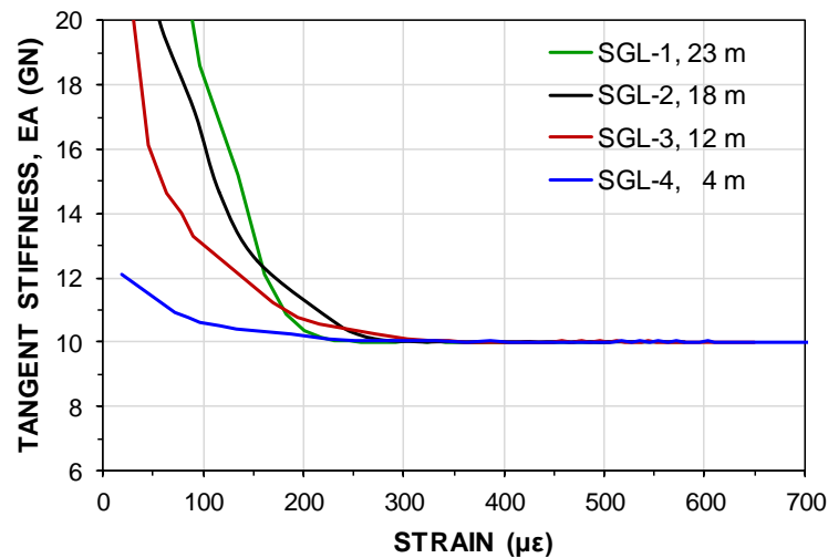
Fig. 8.60 Tangent stiffness for to plastic t-z response.
