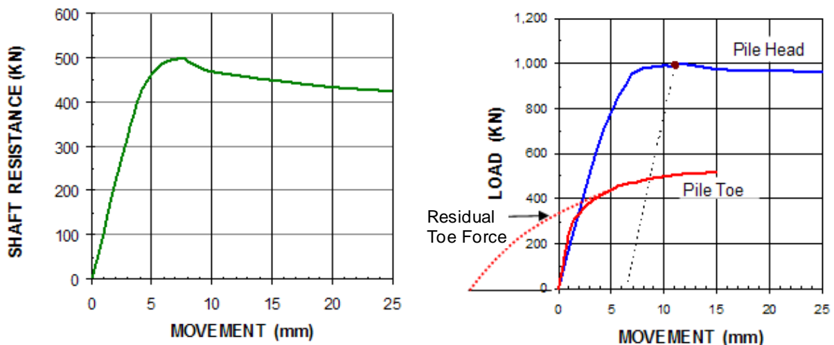
Fig. 7.11 Load-Movement curves for shaft resistance and for total ("Pile Head") and toe resistances.
