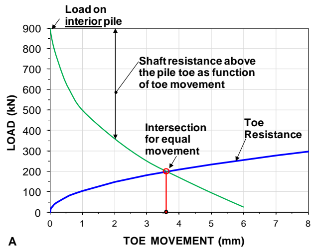
Fig. 8.90A. Load-transfer movement for interior piles
