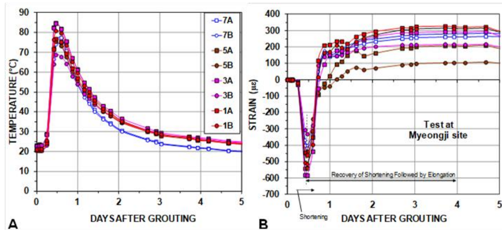
Fig. 8.40 Development of temperature and strain in a 35 m long spun-pile during first 5 days after grouting (reducing strain indicates compression/shortening) (Fellenius et al. 2009)
