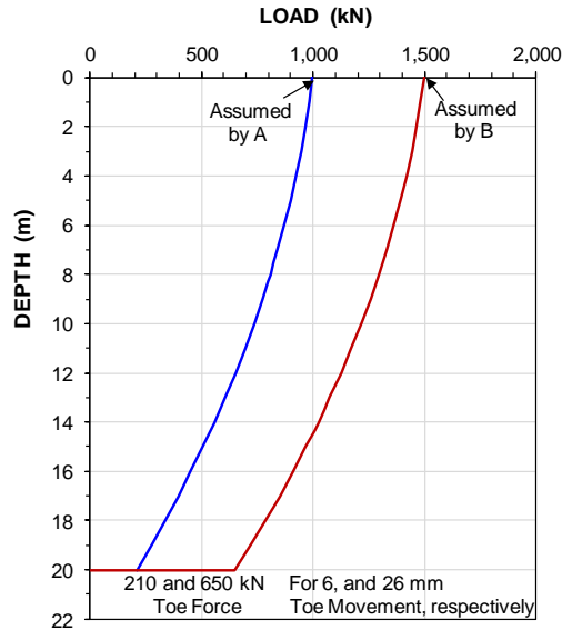
Fig. 8.93 Load distributions as deduced by Persons A and B
