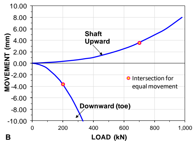
Fig. 8.90B. Simulated BD test
