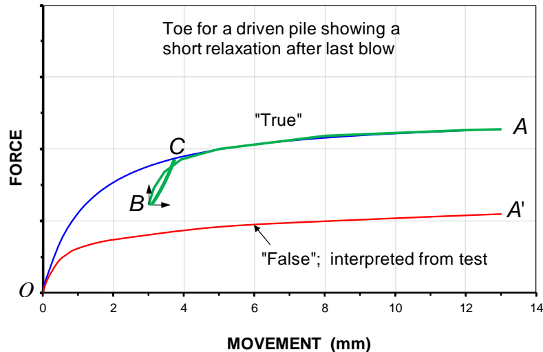
Fig. 8.37. Residual force at the pile toe in case of a driven pile
