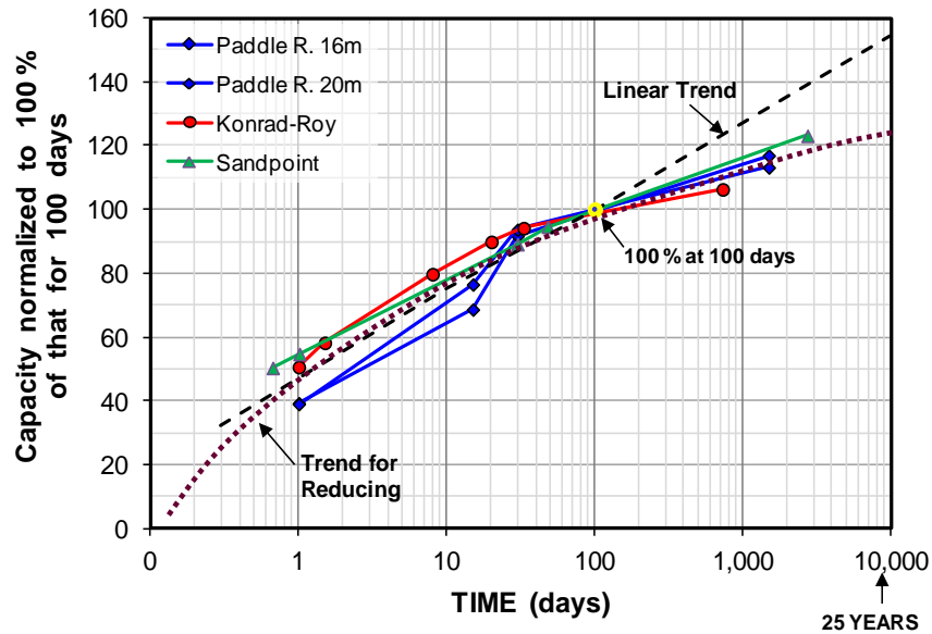
Fig. 7.58 "Capacities" normalized to 100 % of 100-day values
