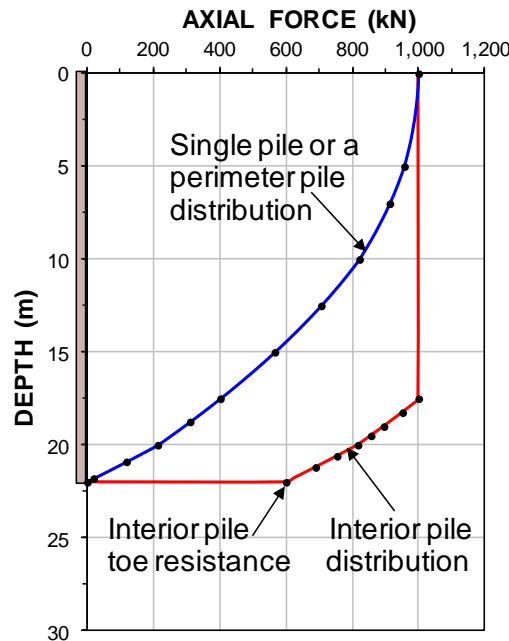
Fig. 7.37. Load distribution for perimeter and interior piles under a flexible raft (same load per pile).
