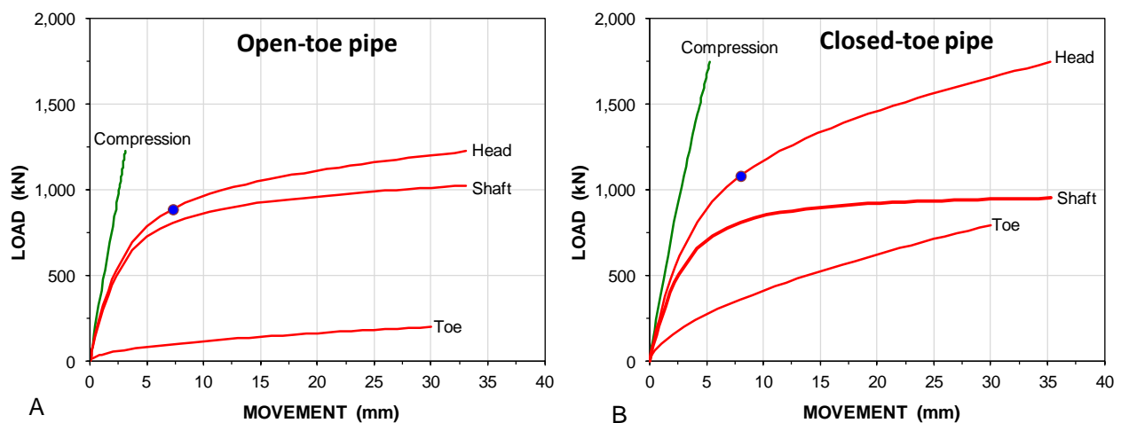
Fig. 7.49 Load-movement curves for a static loading test on (A) open-toe and (B) closed-toe piles
