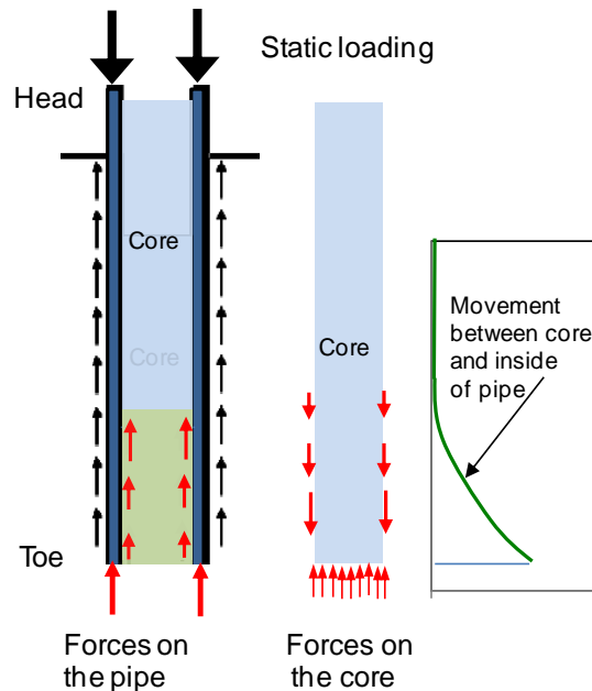
Fig. 7.48 Force vectors in static loading of an open-toe pipe pile with inside soil column, a "core".
