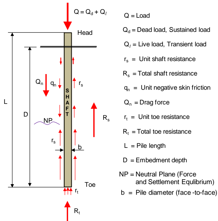
Fig. 7.1 Transfer of load to a pile and from the pile to the soil
