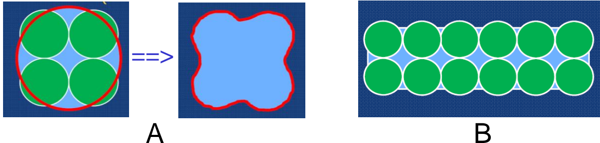
Fig. 7.44 Four piles replacing a single pile and twelve piles replacing a barrette
