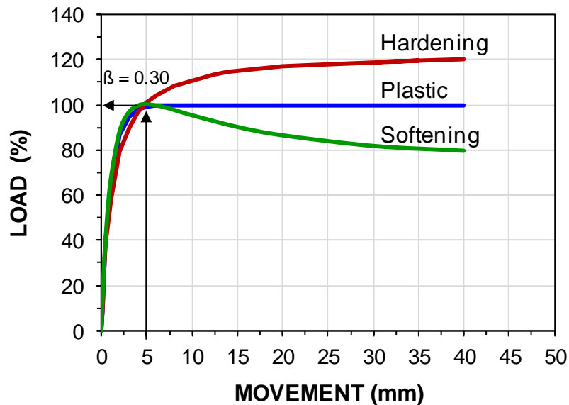
Fig. 8.57 Three alternative t-z functions.
