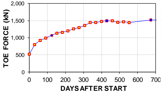
Fig. 7.21A Toe force vs. days after start
