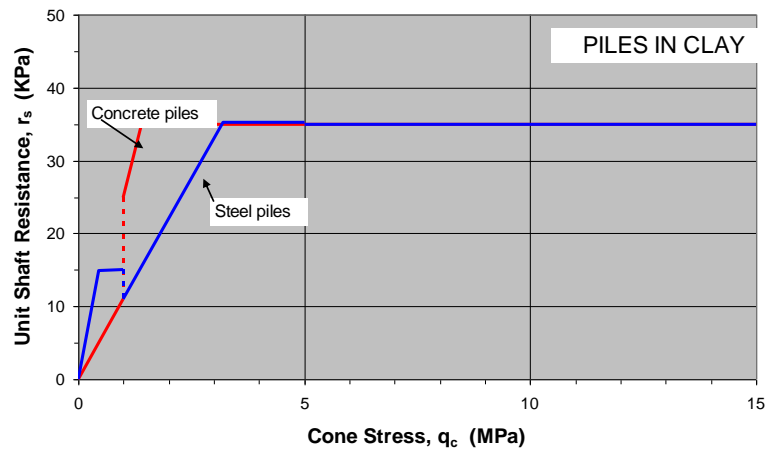
Fig. 7.16 Unit shaft resistance versus cone resistance, q_c , for piles in clay according to the LCPC method.
