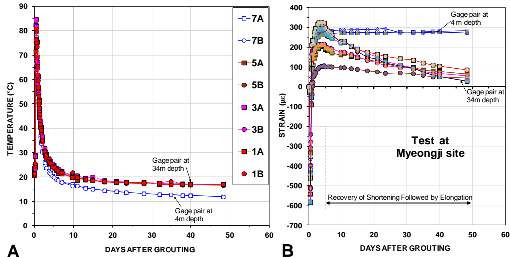
Fig. 8.41 Development of temperature and strain in a 35 m long spun-pile during 50 days after grouting the interior void (Fellenius et al. 2009)
