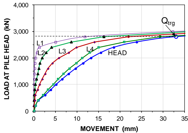
Fig. 8.75 Movements measured for the applied loads Q_{trg} = Target Load.
