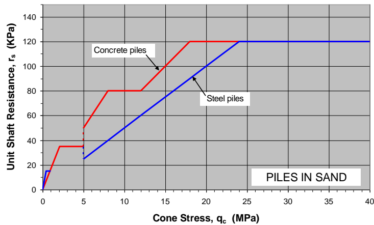
Fig. 7.17 Unit shaft resistance versus cone resistance, q_c , for piles in sand according to the LCPC method.
