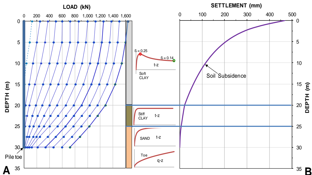
Fig. 7.28 Distributions of axial load in the pile and settlement of the soil around the pile.
