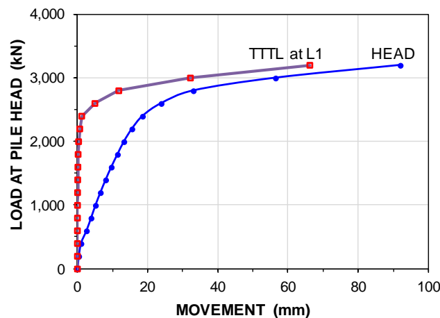
Fig. 8.73 Load-movements for the pile head and pile "toe" (actually for TTL1 at L1).
