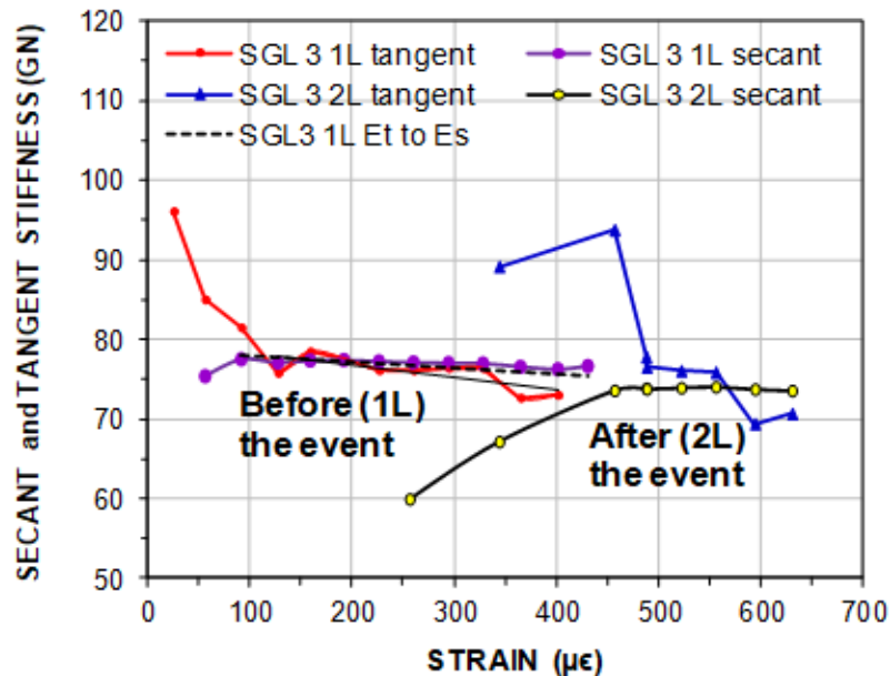
Fig. 8.70 Incremental stiffness ("tangent stiffness") for virgin loading and re-loading; L = 1.0 m.
