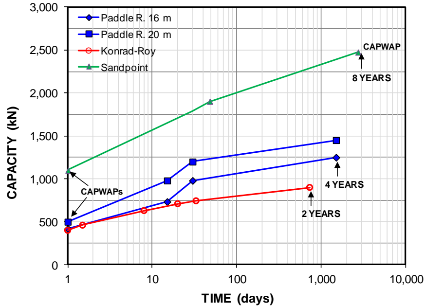
Fig. 7.57 "Capacity" determined at days after driving
