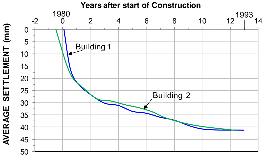
Fig. 7.32 Settlement measured for the two buildings over 13 years.
