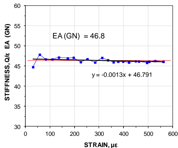
Fig. 8.47 Stiffness vs. measured strain for a not-concreted steel pipe pile (Fellenius 2012)
