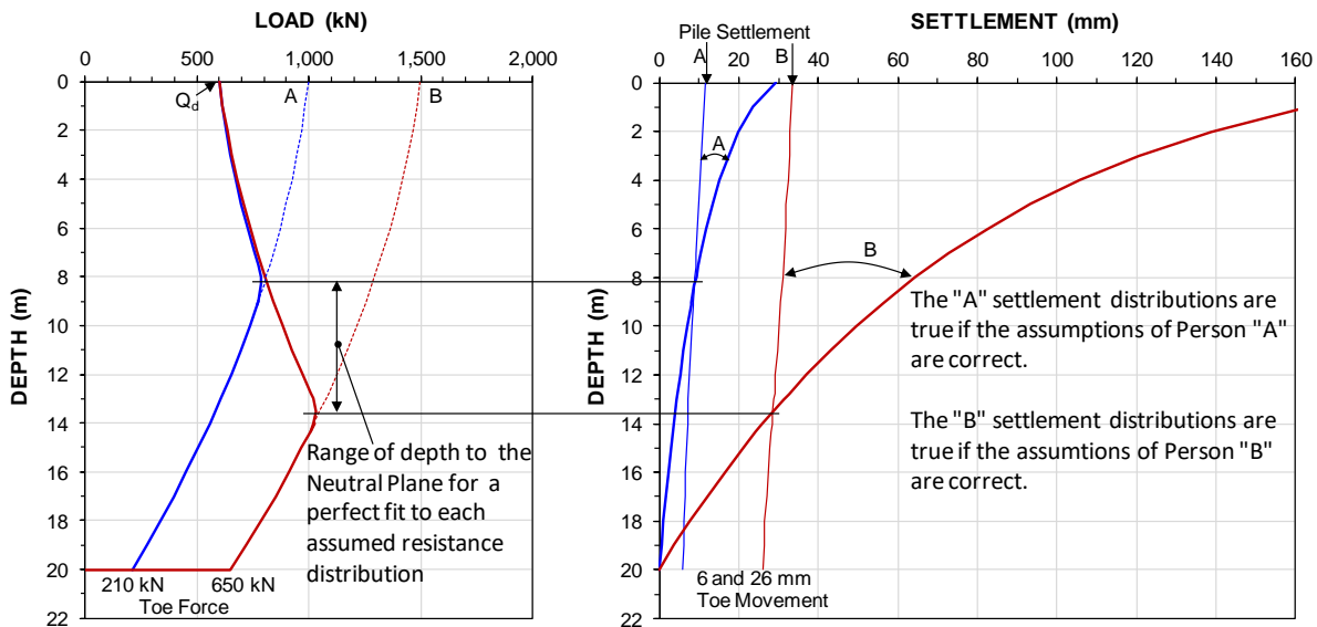
Fig. 8.94 Unified method correlations per the Persons A and B cases
