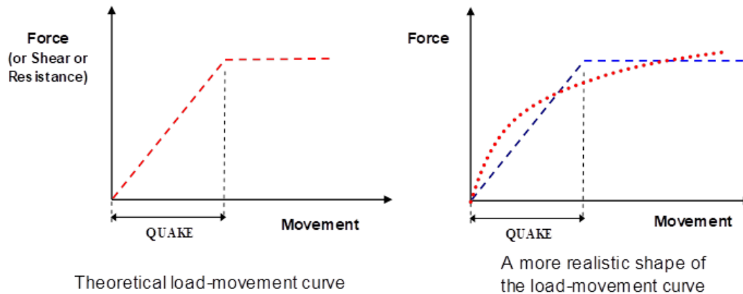
Fig. 9.8 Development of soil resistance to pile movement (q-z curves).
