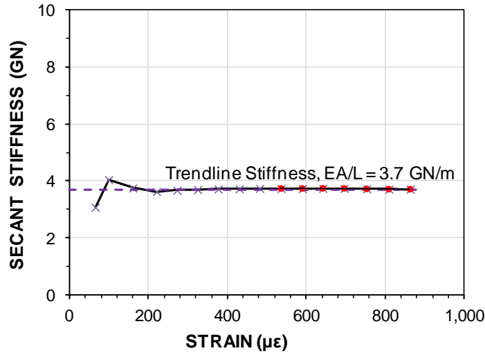
Fig. 8.78 Secant stiffness, E_s A/L , at L4.
