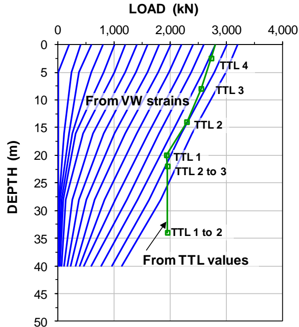
Fig. 8.80. Distributions load in VW-gages and from telltales at the 2,800-kN Target Load.
