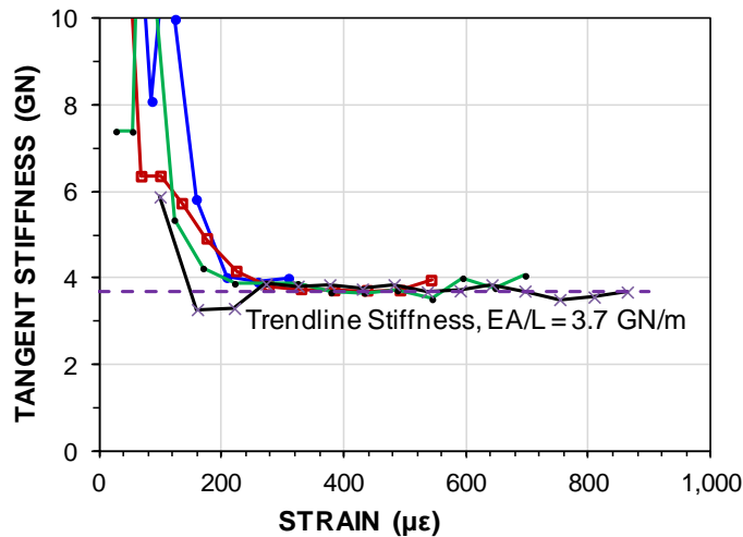
Fig. 8.79. Tangent stiffness.
