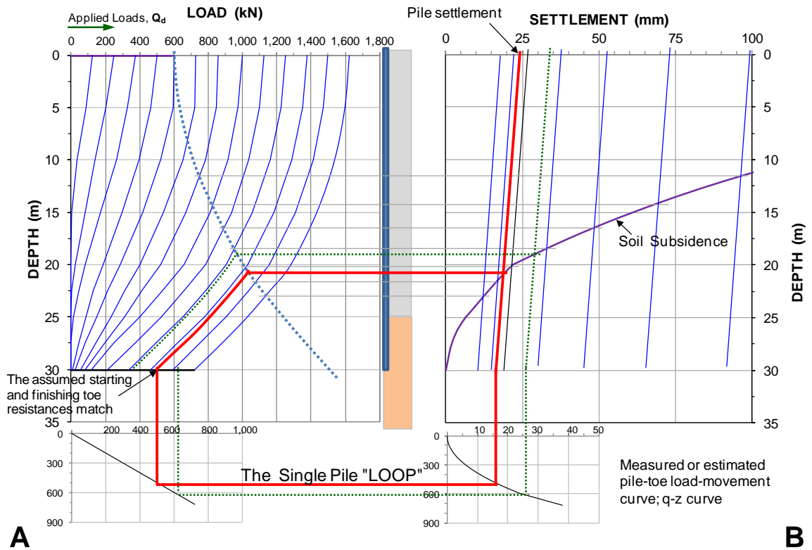
Fig. 7.31 Final match between starting and finished toe resistance and determining the pile settlement.
