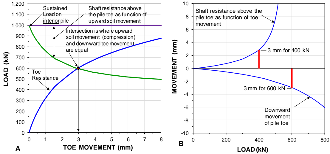
Fig. 7.36. The process for determining the load-transfer toe-movement for interior piles.
