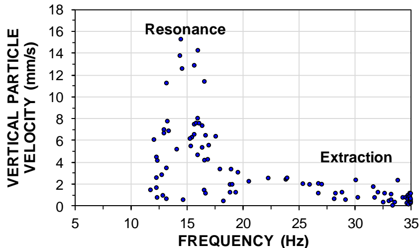
Figure 10.15 Ground vibration velocity during probe penetration, compaction, and extraction measured at 4 m distance from the compaction probe (Massarsch and Fellenius 2005).
