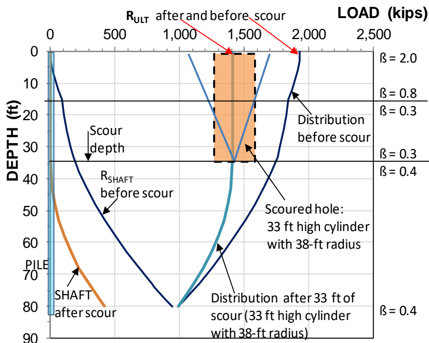
Fig. 7.60 Load distributions at "capacity" before and after-scour
