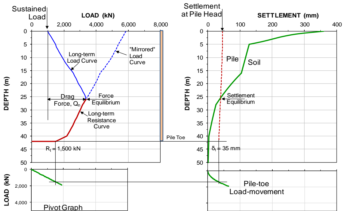
Fig. 8.89. Load and settlement distributions for the long-term conditions of the single 600-mm pile.
