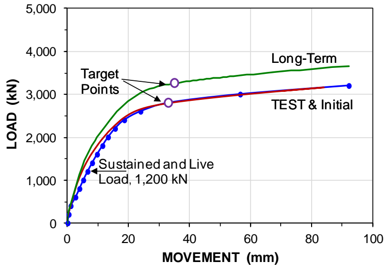
Fig. 8.86. Pile-head load-movements at the test (initial) and long-term conditions.
