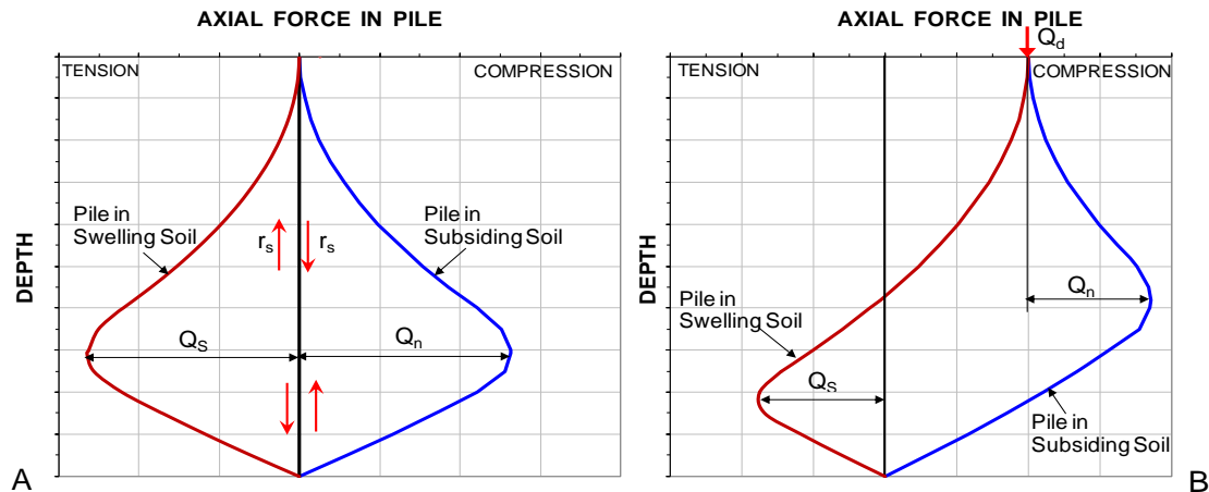
Fig. 7.25 Load distribution for a pile in swelling soil underlain by a non-swelling soil Fig. 7.25 A Shaft shear distribution Figure 7.25 B Load distribution
