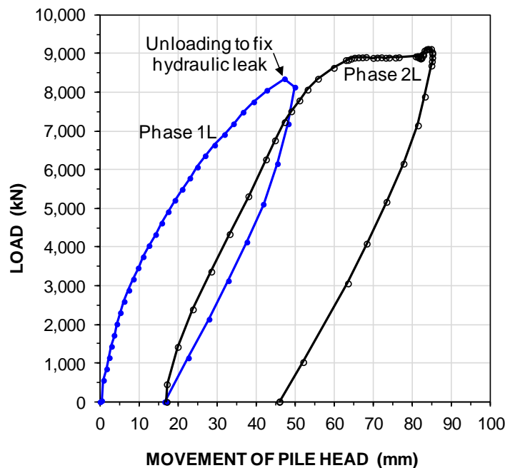
Fig. 8.63 Pile-head load-movement for the 600-mm cylinder pile with unloading-reloading event.
