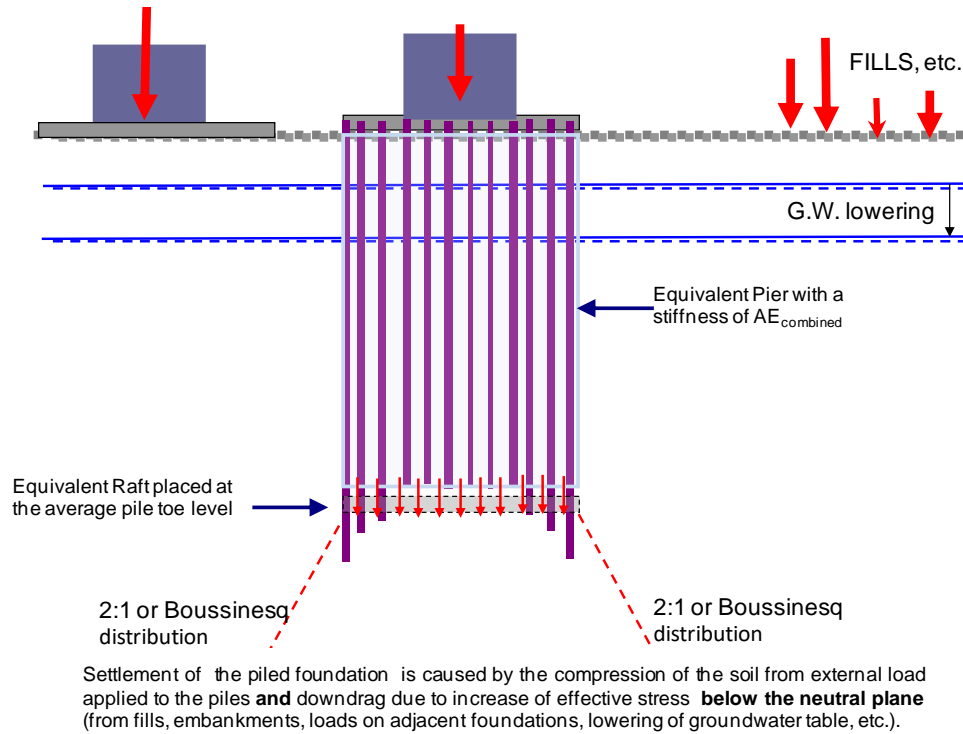
Fig. 7.55 Lengthening of perimeter to minimize downdrag.
