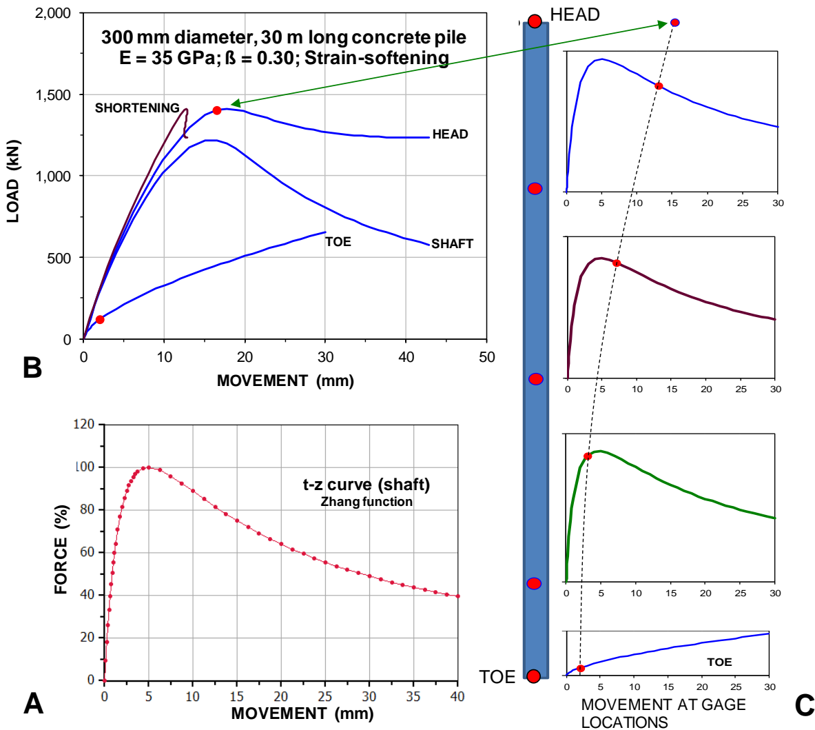
Fig. 7.10 Load-movement curves and t - z curves
