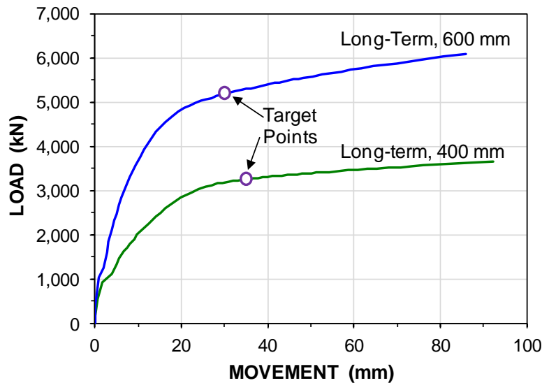
Fig. 8.88. Pile-head load-movements for long-term conditions of the 400-mm and 600-mm piles.
