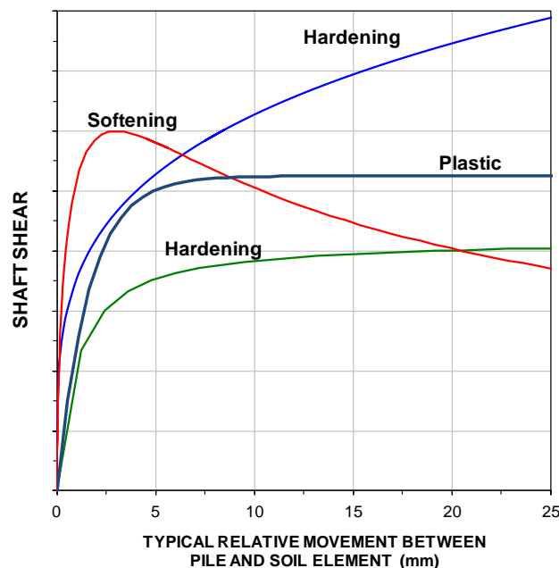
Fig. 8.9 Typical resistance versus movement curves
