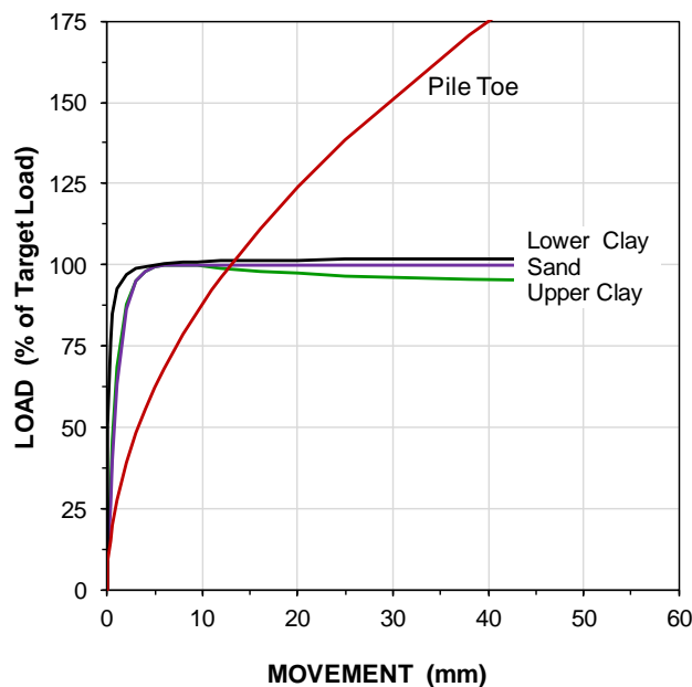
Fig. 8.84 Compilation of all four t-z curves used as input for the load-movement measurements.
