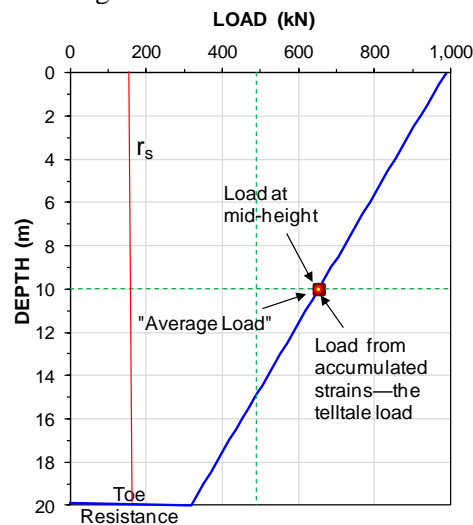
Fig. 8.20 Load distribution for constant unit shaft resistance.
