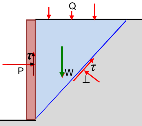
Fig. 11.2 Earth Stress; a sliding soil wedge retained by a wall
