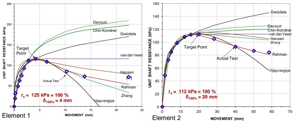
Fig. 8.19. Comparison of best-fit functions to two actual records of unit strain-softening shaft resistance (kPa) vs. movement (mm). Data from Bohn et al. 2017.
