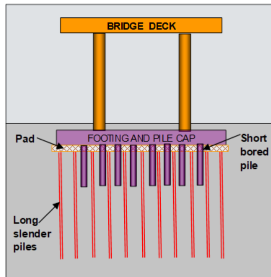
Fig. 7.43 Piled pad foundations for the Golden Ears Bridge piers. The short bored piles carry lateral forces, the long slender piles carry the structure (after Sampaco et al. 2008)
