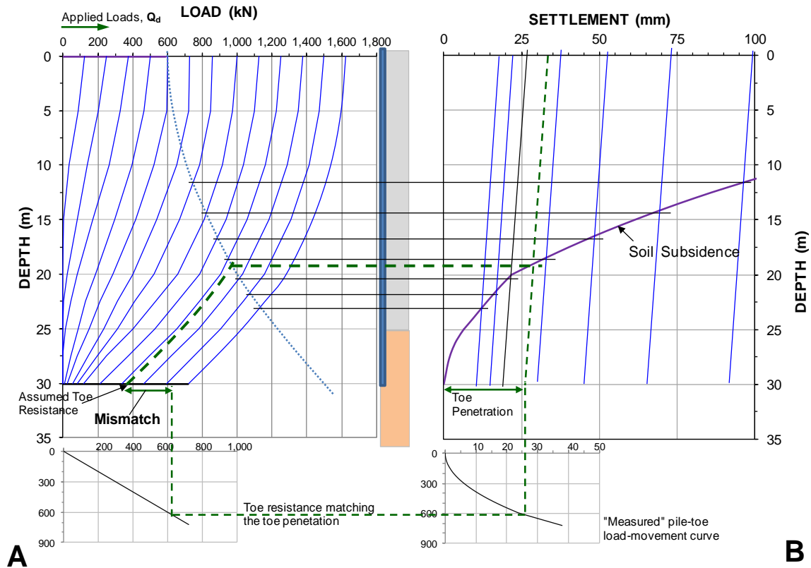
Fig. 7.30 First attempt to find the true neutral plane resulting in "mismatch".
