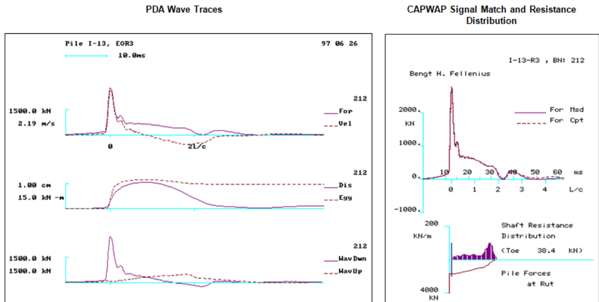
Fig. 9.17 Example of a routine PDA and CAPWAP summary sheet: Table and graph
