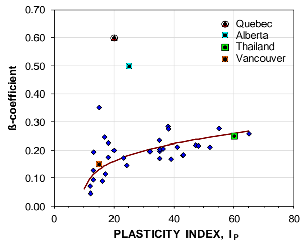
Fig. 7.5 Beta-coefficient for piles in clay versus plasticity index, I_p . (Data from Clausen et al. 2005 with results from four cases added; Fellenius 2006).
