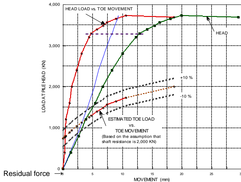
Fig. 8.22 The same test data as shown in Fig. 8.21 with the results of analysis of the load-movement of the pile toe. The results from a static loading test on an adjacent pile instrumented with strain-gages indicated that the shaft resistance would be about 2,000 kN (Fellenius 1999).
