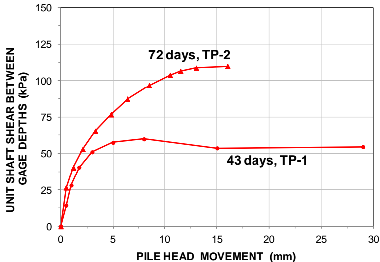
Fig. 7.56 Shaft resistance vs. average gage movement on two occasions after construction (Data from Teparaska 2015)
