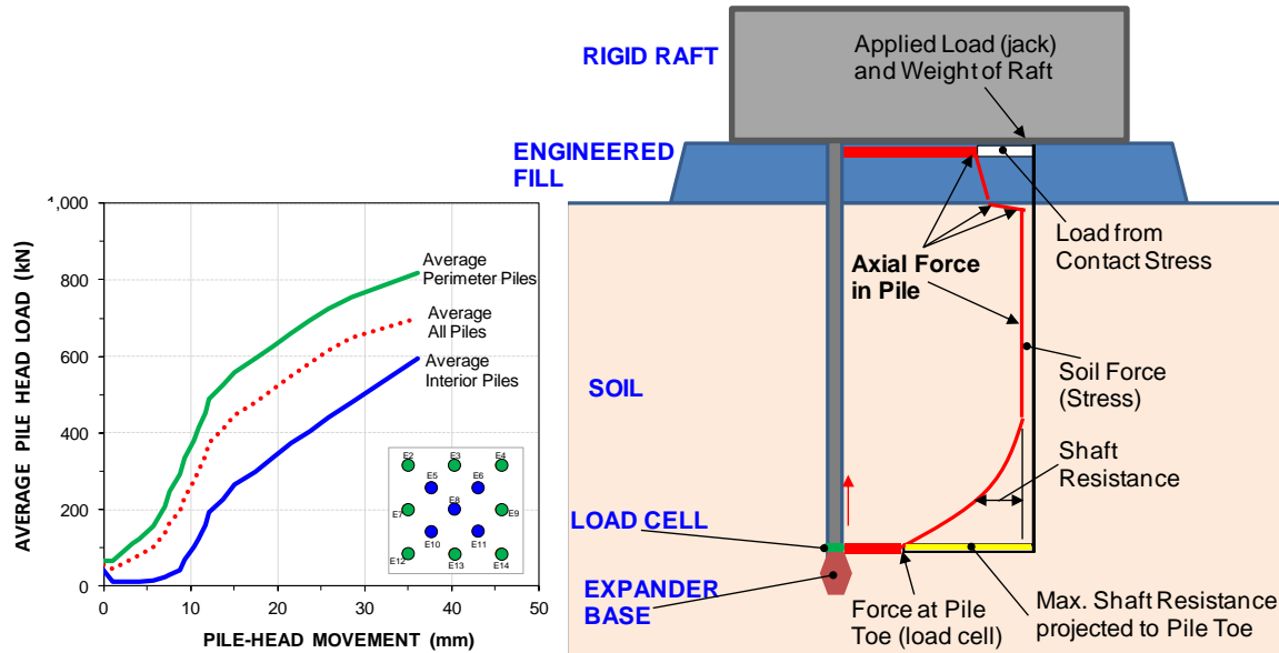
Fig. 7.35 Perimeter pile-head load-movement curves and distribution of axial force and maximum load
