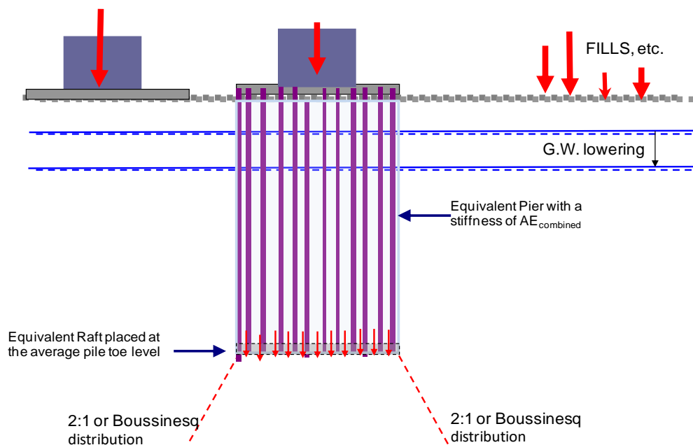
Fig. 7.39. The equivalent raft for calculation of settlement below the pile toe level.
