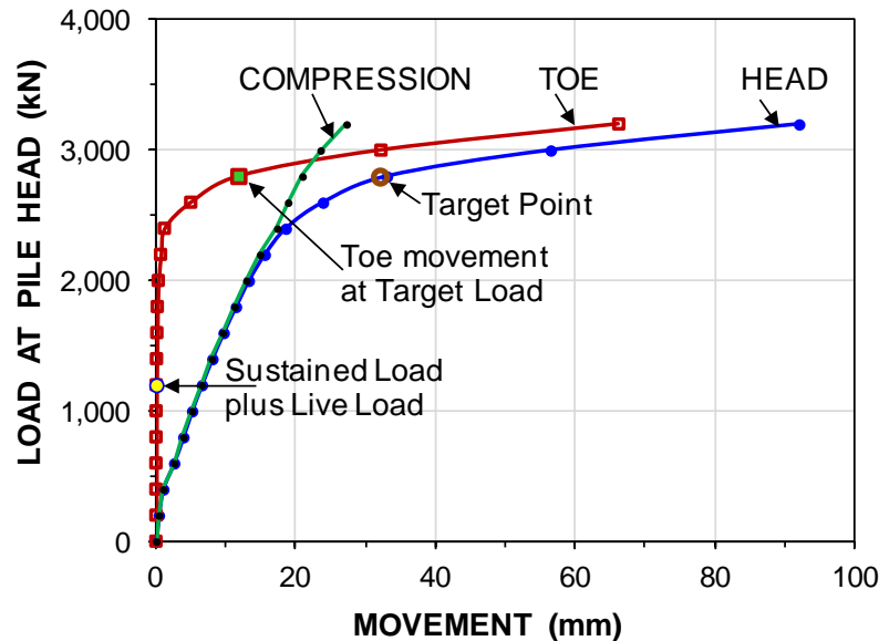
Fig. 8.77 Load-movements for the pile head and pile "toe" with the pile compression and Target Point (Pile-head load-movement).
