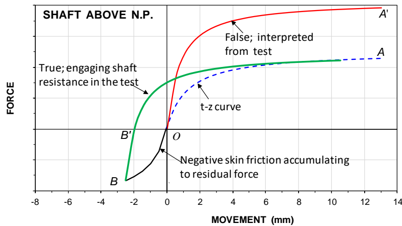
Fig. 8.35. The development of "false" resistance from downdrag
