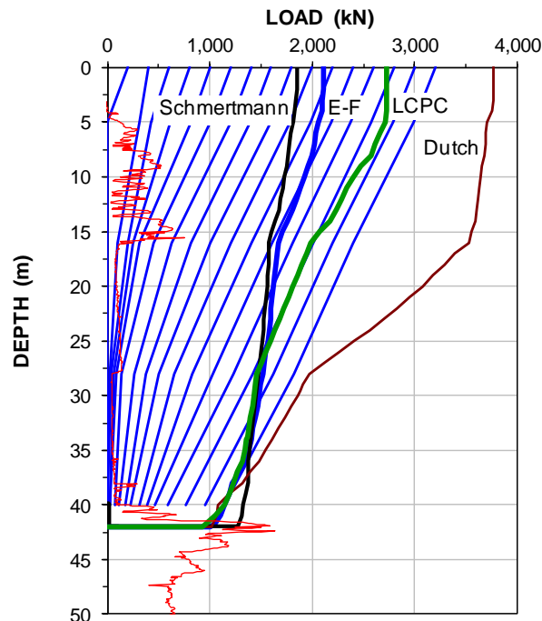
Fig. 8.81. Load distributions from VW records compared to distributions per CPT/CPTU methods.
