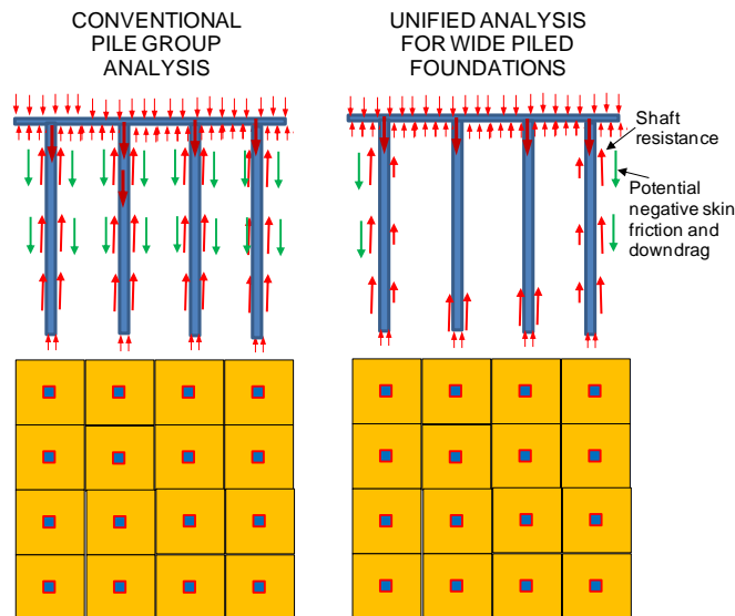
Fig. 7.41 Comparison between conventional and unified method of analysis of a wide pile group.
