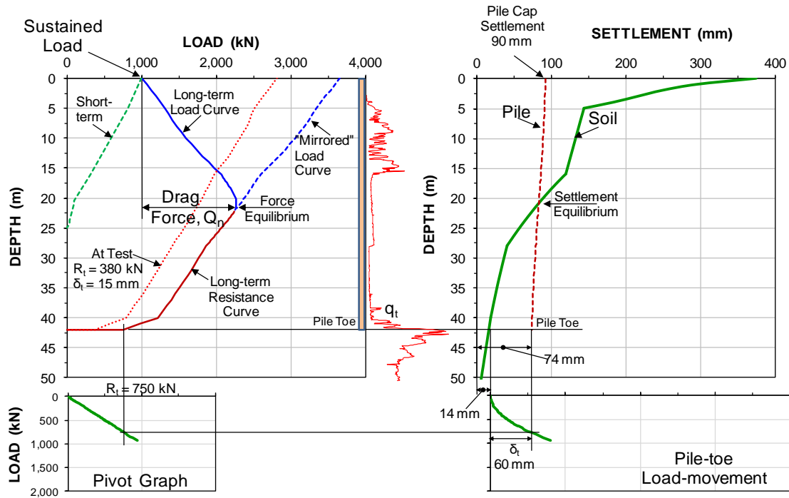
Fig. 8.87. Load and settlement distributions for the long-term conditions of the single 400-mm pile.
