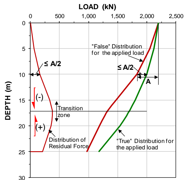
Fig. 8.38. Procedure for estimating distribution of residual force and "true" resistance
