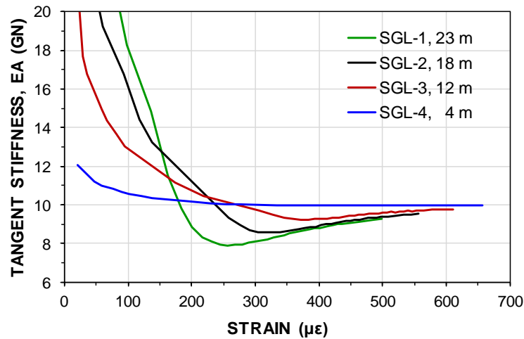
Fig. 8.62 Tangent stiffness for softening t-z response; element length.
