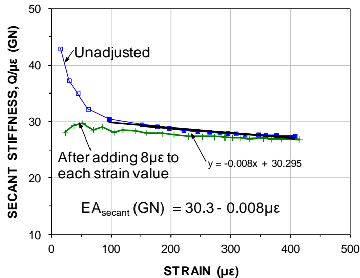
Fig. 8.50 Secant stiffness ( Q/\mu\epsilon ) vs. measured strain for a 900-mm bored pile (data from GeoOptima 2011)
