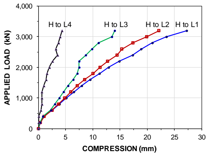
Fig. 8.76 Pile compression above gage levels for the applied load determined from subtracting TTL movement from pile-head movement. The label "H to L#" means compression between pile head and telltale end".
