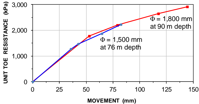
Fig. 7.7 Unit toe resistance measured in two bored piles with different diameters constructed to different depths at the same site with different diameter (Data from Fellenius and Nguyen 2013).
