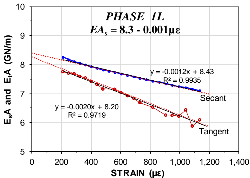
Fig. 8.65 Secant and tangent stiffness plots from SGL-12 close to the pile-head
