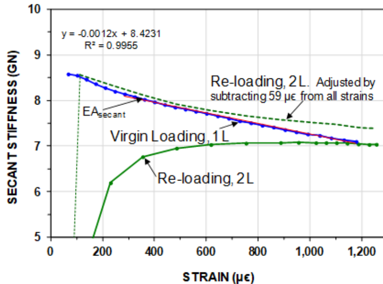
Fig. 8.66 Secant stiffness plot of the from the near-the pile-head gage records
