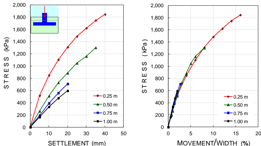
Fig. 6.7 Results of static loading tests on square footings in well graded sand (Data from Ismael, 1985)
