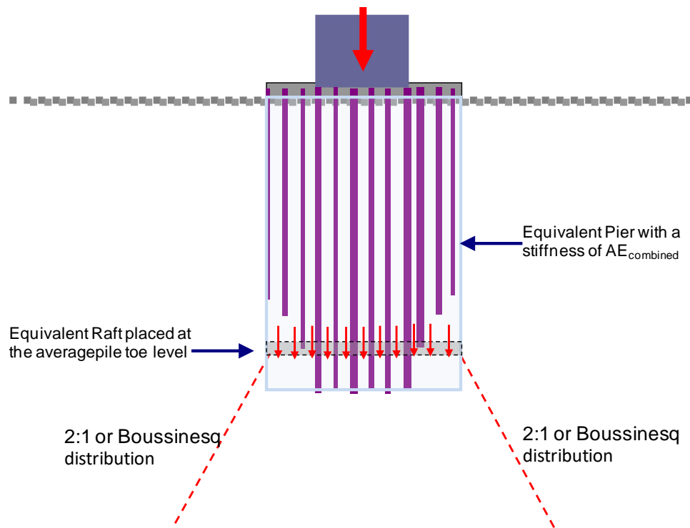
Fig. 7.54 Shortened perimeter piles to reduce differential settlement and load differences.
