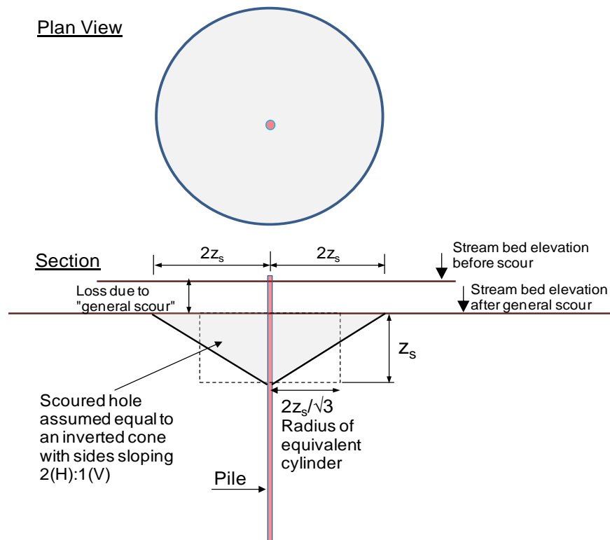
Fig. 7.59. Scour configuration according to the FHWA Manual
