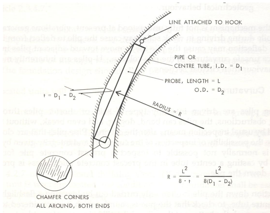
Fig. 7.51 Principle of the curvature probe
