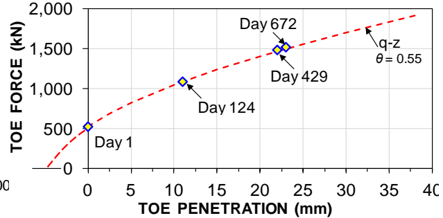
Fig. 7.21B Toe force vs. toe penetration
