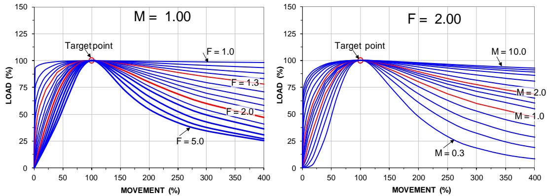
Fig. 8.17. Rahman function for t-z shaft shear force vs. movement.
