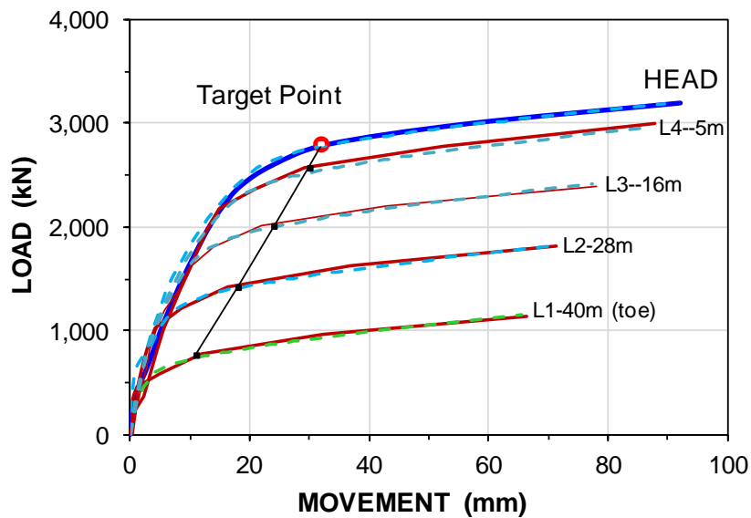
Fig. 8.85. Measured and fitted load-movement curves of pile head and gage levels.
