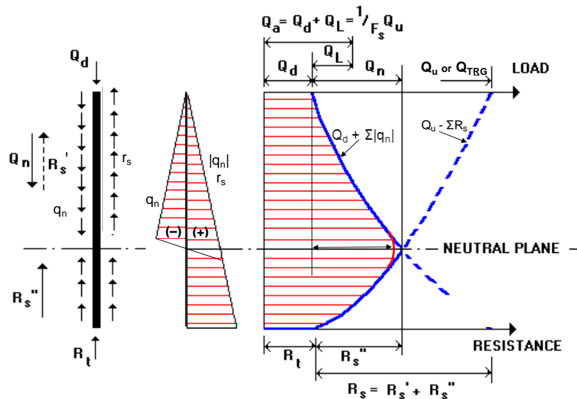
Fig. 7.23 Construing the Force Equilibrium Neutral Plane for a target load, Q_{trg}
