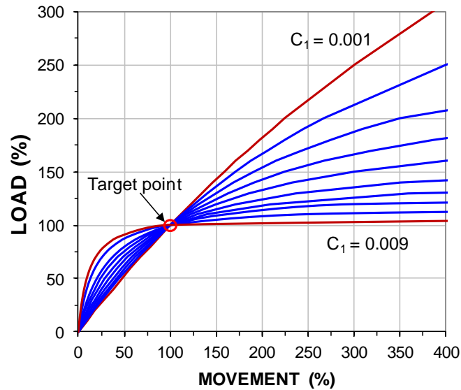
Fig. 8.12 The hyperbolic (Chin-Kondner) for t-z shaft shear force vs. movement
