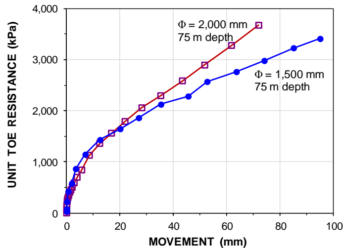
Fig. 7.8 Unit toe resistance measured in two bored piles with different diameter (1,500 and 2,000 mm) constructed to the same 75-m depth (Data from Fellenius and Nguyen 2014).
