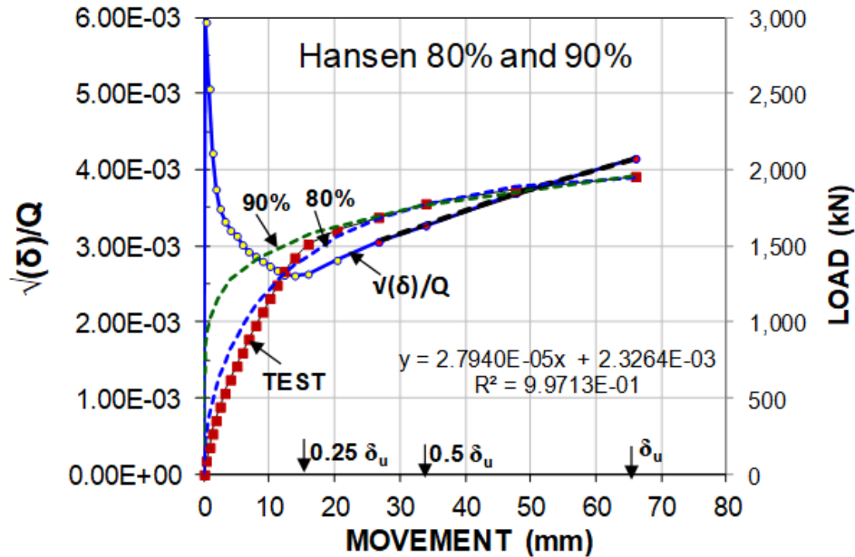
Fig. 8.2 Hansen's Plot for the 80 and 90 percent criteria
