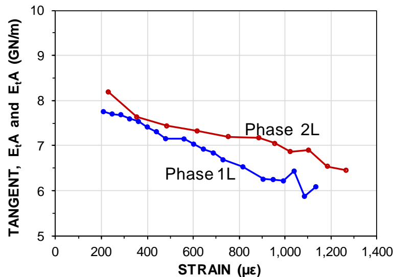
Fig. 8.67 Incremental stiffness ("tangent stiffness") for virgin loading and re-loading
