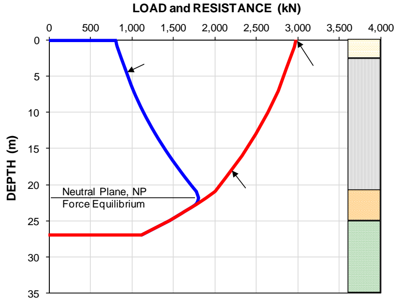
Fig. 7.9 Load-transfer and resistance curves and force-equilibrium Neutral-Plane
