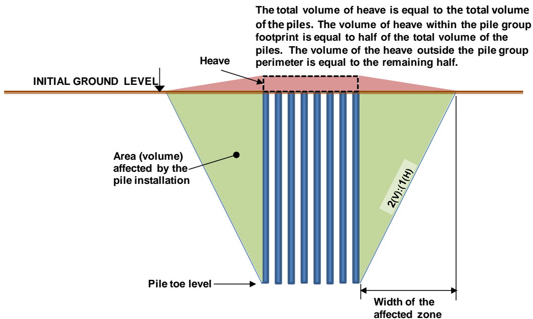
Fig. 7.53 Amount of heave and zone affected by driving a group of piles into soft clay
