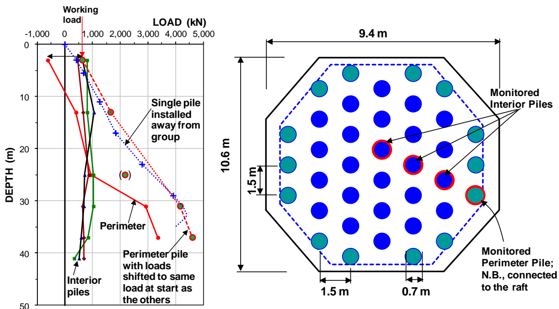
Fig. 7.34 Axial pile loads measured 4.5 years after construction (Okabe 1977)
