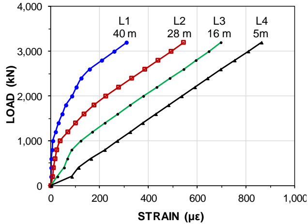
Fig. 8.74 Strains measured for the applied loads.
