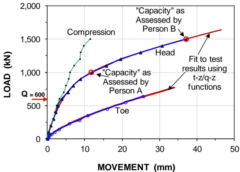
Fig. 8.91. Pile-head load-movement for the example pile with two different capacity assessments. The red curve is the result of a simulation of the test curve using UniPile 5.
