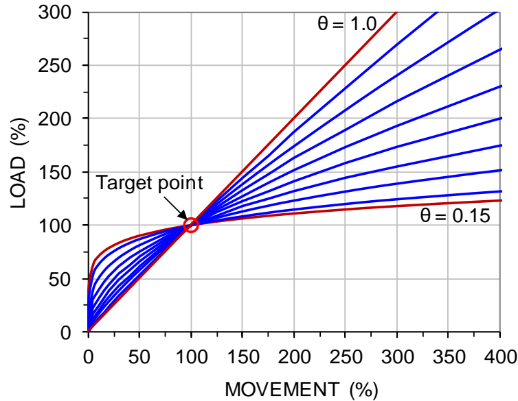
Fig. 8.11 Gwizdala Function for t-z shaft shear force vs. movement
