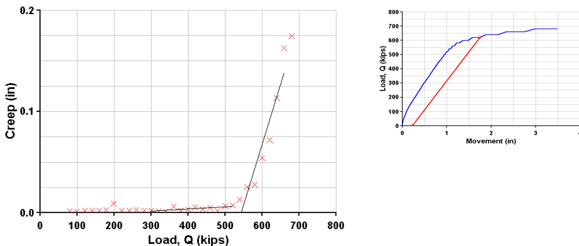
Fig. 8.6 Plot for determining the creep limit
