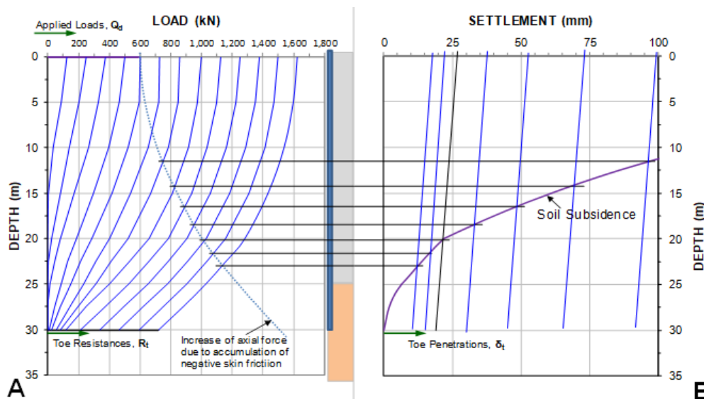
Fig. 7.29 Potential force and settlement equilibrium lines added to Fig. 7.28 (Fellenius 2017; 2019).
