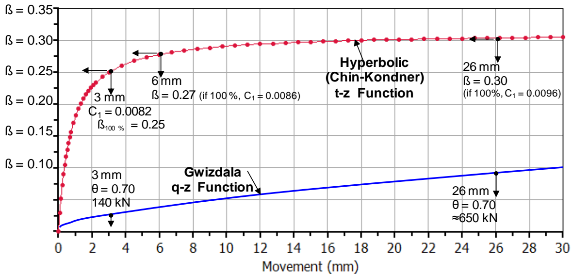
Fig. 8.92. The t - z and q - z response of the test pile.
