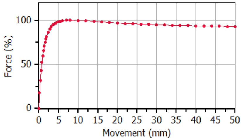
Fig. 8.83. The Zhang strain-softening t-z curve used as input for the 5.0 m thick upper soft clay layer.
