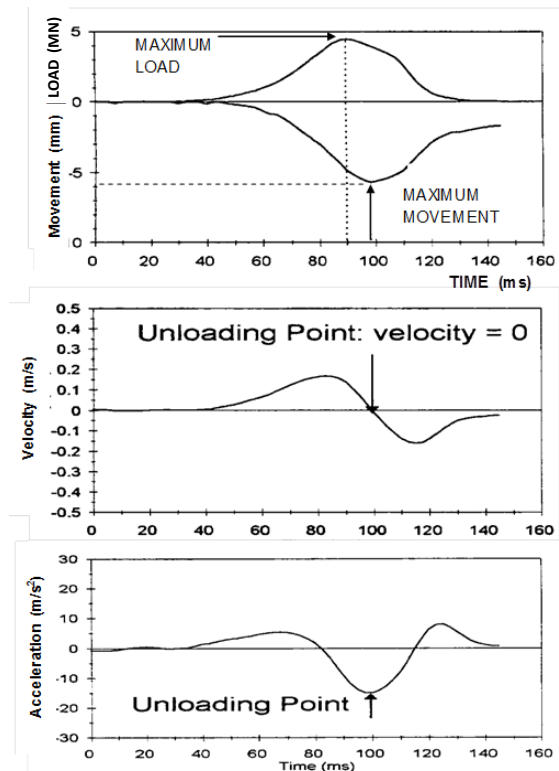
Fig. 9.22 Load, movement, velocity, and acceleration versus time from a Statnamic test (Bermingham et al. 1993; used with permission)
