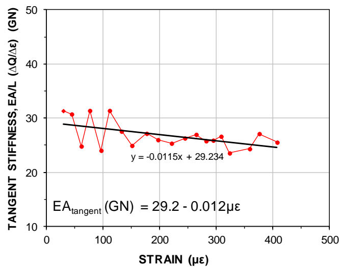
Fig. 8.51 Tangent stiffness determined from the strain records unaffected by shaft resistance.
