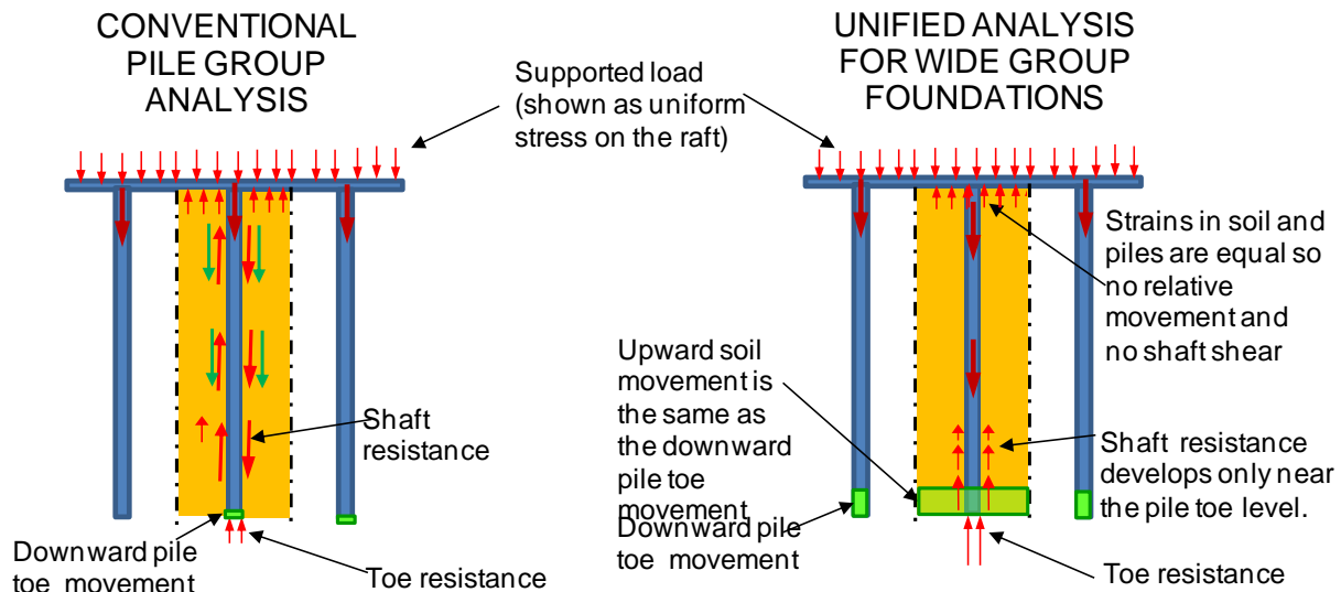
Fig. 7.42 Comparison between conventional and unified methods of analysis of interior piles
