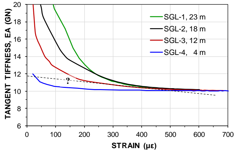
Fig. 8.61 Tangent stiffness, for hardening t-z response.
