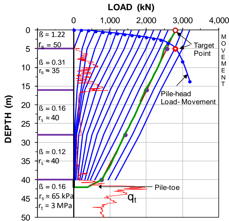
Fig. 8.82. Load distributions from VW-gages and UniPile effective stress analysis.
