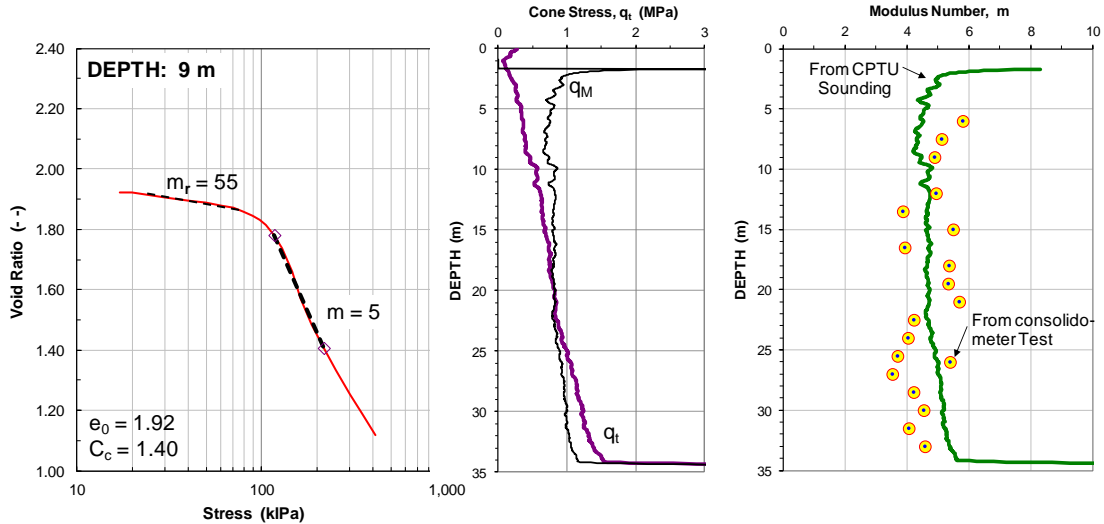
Fig. 4 Results of a consolidometer test from 9 m depth
