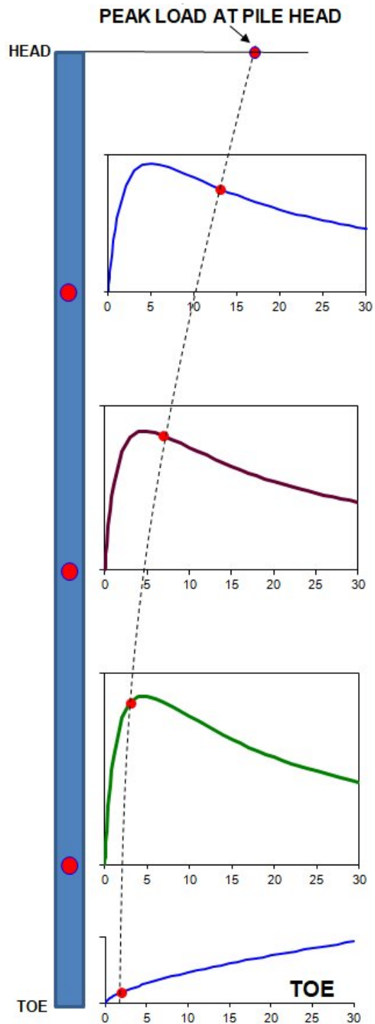
Fig. 7. Distribution of axial force with depth
