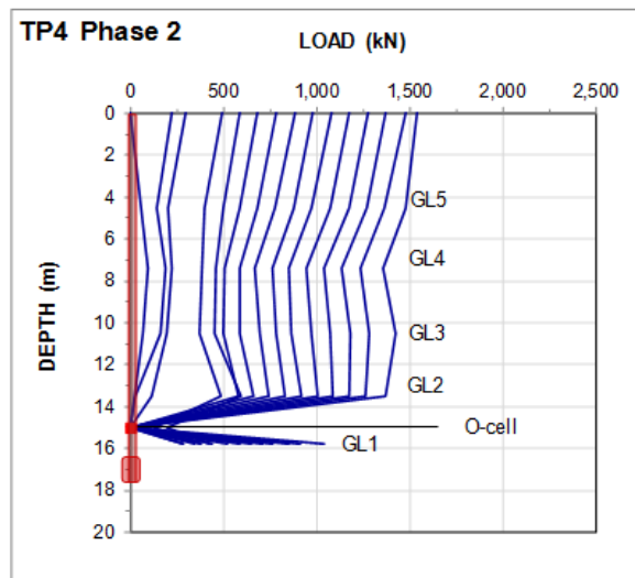
Fig. 20 Pile TP4 Phase 2 Load distribution
