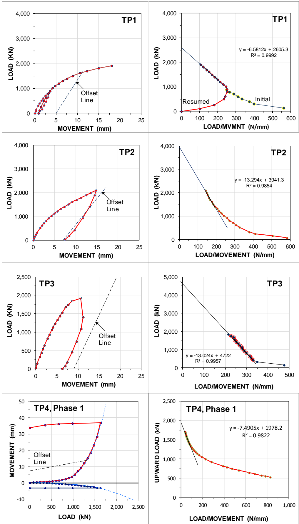
Fig. 8 TP1-TP4 Load-movement curves and Decourt constructions
