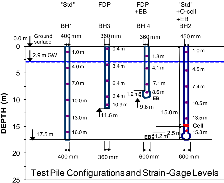
Fig. 5 Vertical view of the test site
