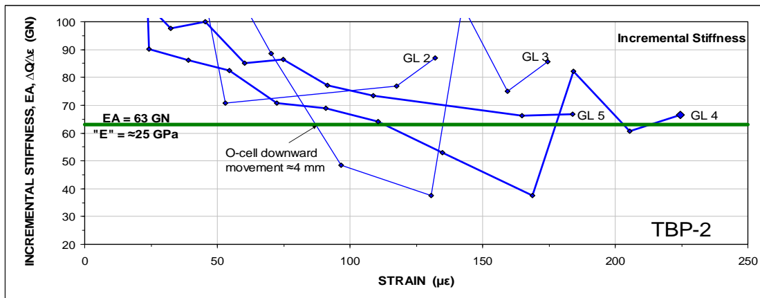
Figure 7 Incremental stiffness plot of the strain-gage measurements from Pile TBP-2
