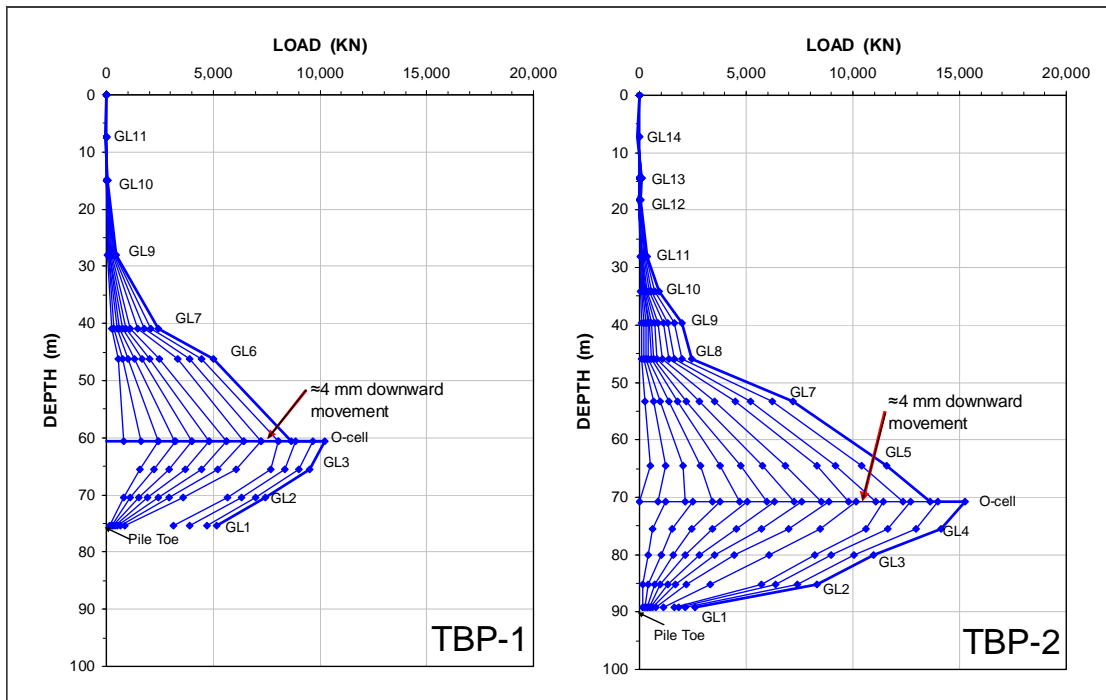
Figure 8 Load distribution in Piles TBP-1 and TBP-2
