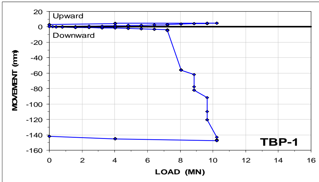
Figure 4 Load-movement measured for Pile TBP-1
