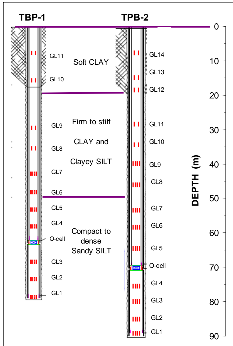
Figure 3. Schematics of the O-cell test piles
