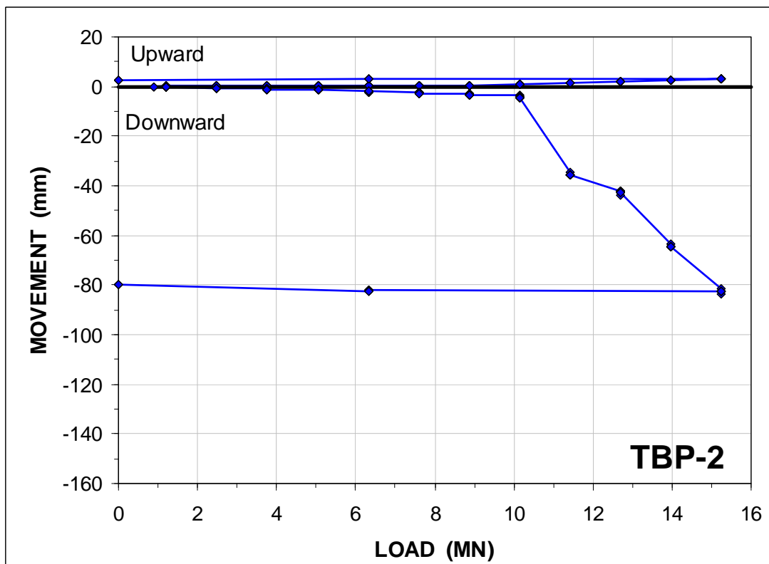
Figure 5 Load-movement measured for Pile TBP-2
