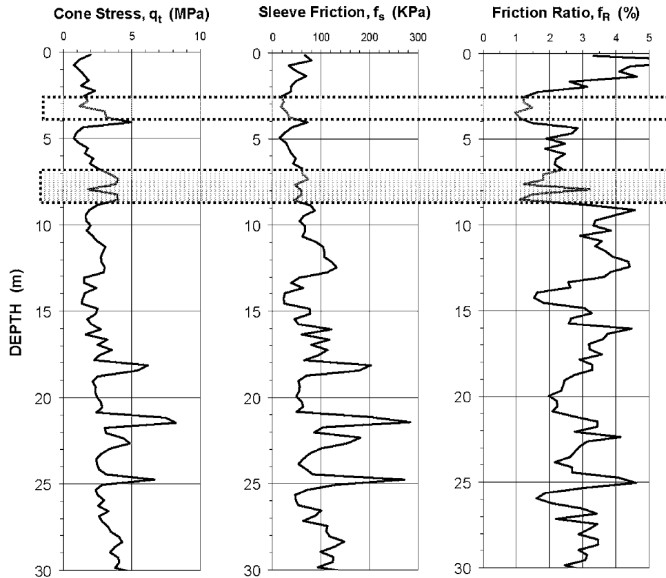
Fig. 1. CPT profile from example site. Two zones surrounded by dashed lines are identified as consisting of sand and silty sand and are considered susceptible to liquefaction during design earthquake.
