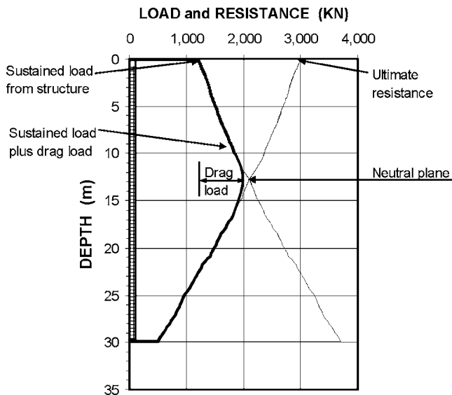
Fig. 2. Distribution of load and resistance along pile before liquefaction
