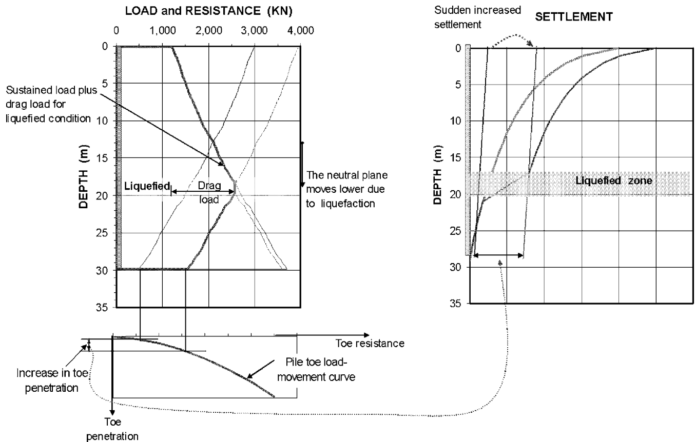
Fig. 4. Distribution of load and resistance during liquefaction below neutral plane and settlement before and after liquefaction event
