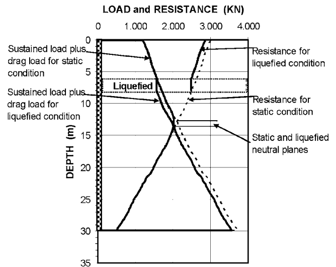
Fig. 3. Distribution of load and resistance during liquefaction above neutral plane
